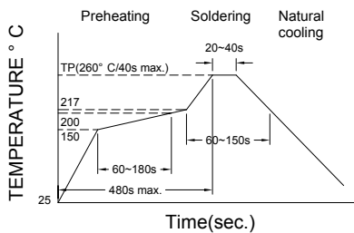
Figure 1. Re-flow Soldering
